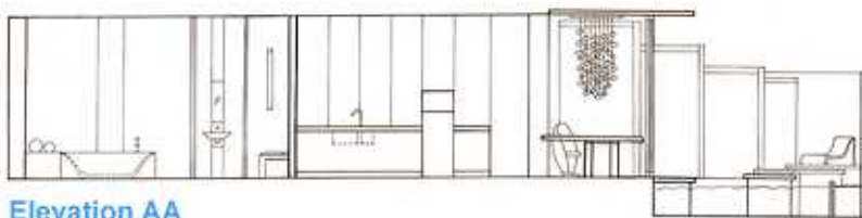
Elevation AA
